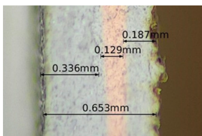
Cross-section of paint flake
